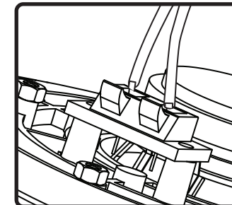
5. Insert signal wire in to spring terminal.
