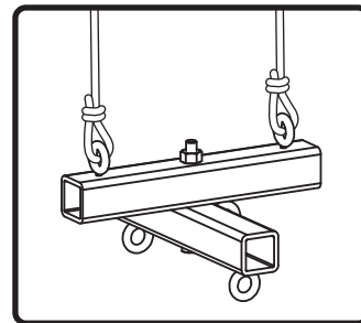
4. Hang the Allen Products One-Way-Array bracket from the structure. Installation location and hanging hardware must be sufficiently strong to reliably hold the speaker. See Allen Products installation manual for more details.
