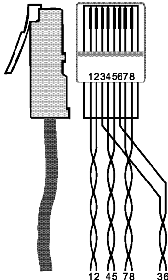
Figure 8: RJ-45 PINOUT
