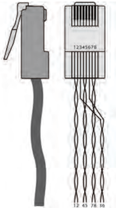
Figure 15: CAT 5 PINOUT
