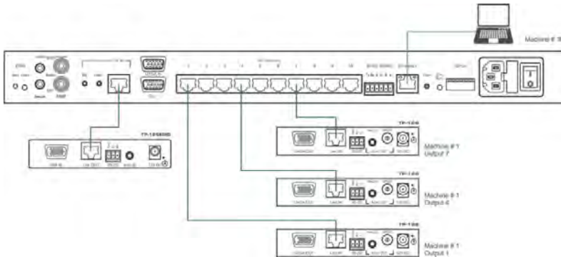
Figure 9: Control via the Ethernet
