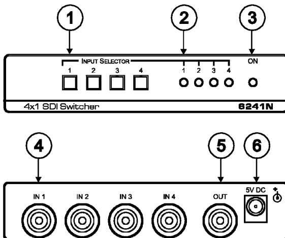
Figure 1: 6241N 4x1 SDI Switcher Functions
