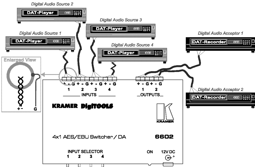
Figure 2: Connecting the 6602 4x1 AES/EBU Switcher / DA
