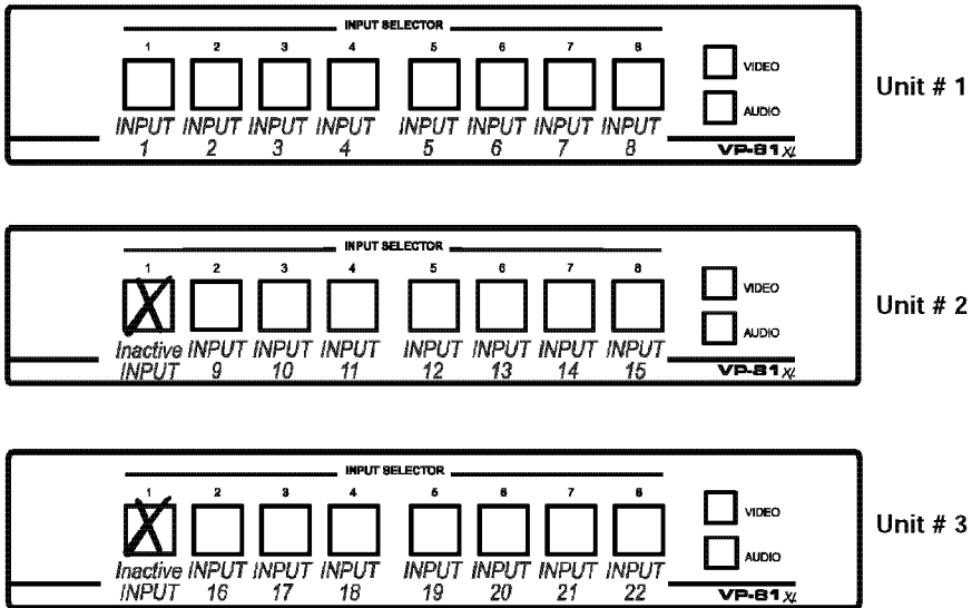
Figure 13: Operating a 22x1 XGA / Audio Switcher (Three Looped VP-81xl Units)
