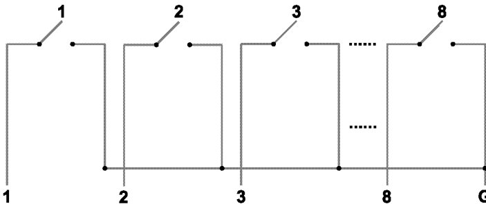
Figure 11: Connecting a Remote Mechanical Switcher Unit to the VP-81xl
