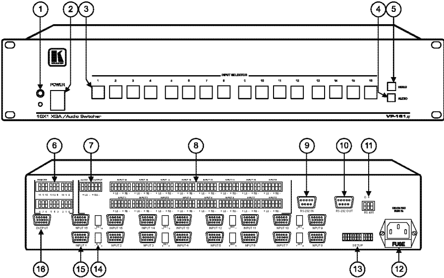
Figure 2: VP-161xl 16x1 XGA / Audio Switcher
