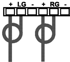
Figure 5: Connecting the Unbalanced Stereo Audio Input/Output
