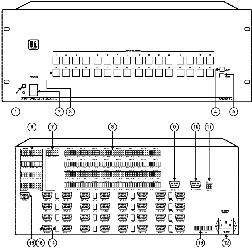
Figure 3: VP-321xl 32x1 XGA / Audio Switcher
