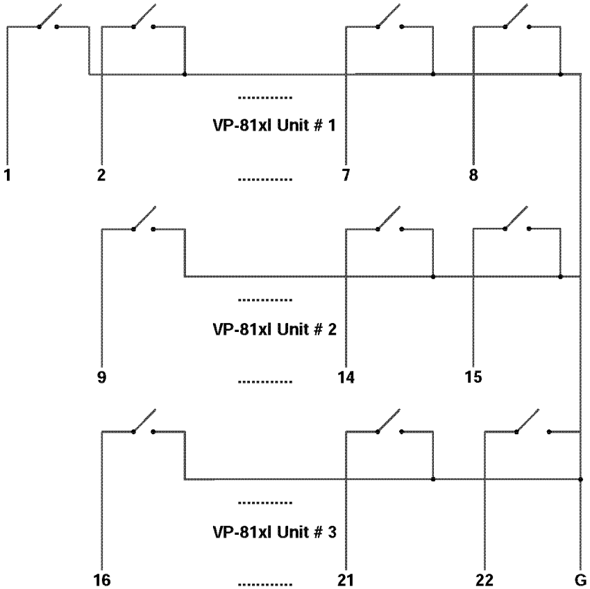
Figure 12: Connecting a Remote Unit to a Cascaded Set of Three VP-81xl Units
