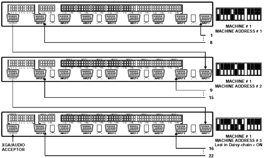
Figure 10: An Interconnected Set of Three Looped VP-81xl Units (Video Connections Shown)
