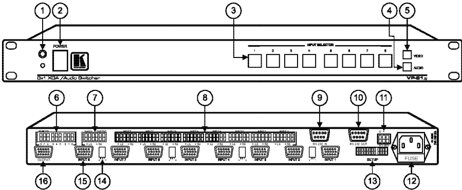
Figure 1: VP-81xl 8x1 XGA / Audio Switcher
