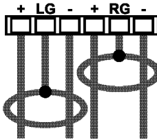
Figure 4: Connecting the Balanced Stereo Audio Input/Output
