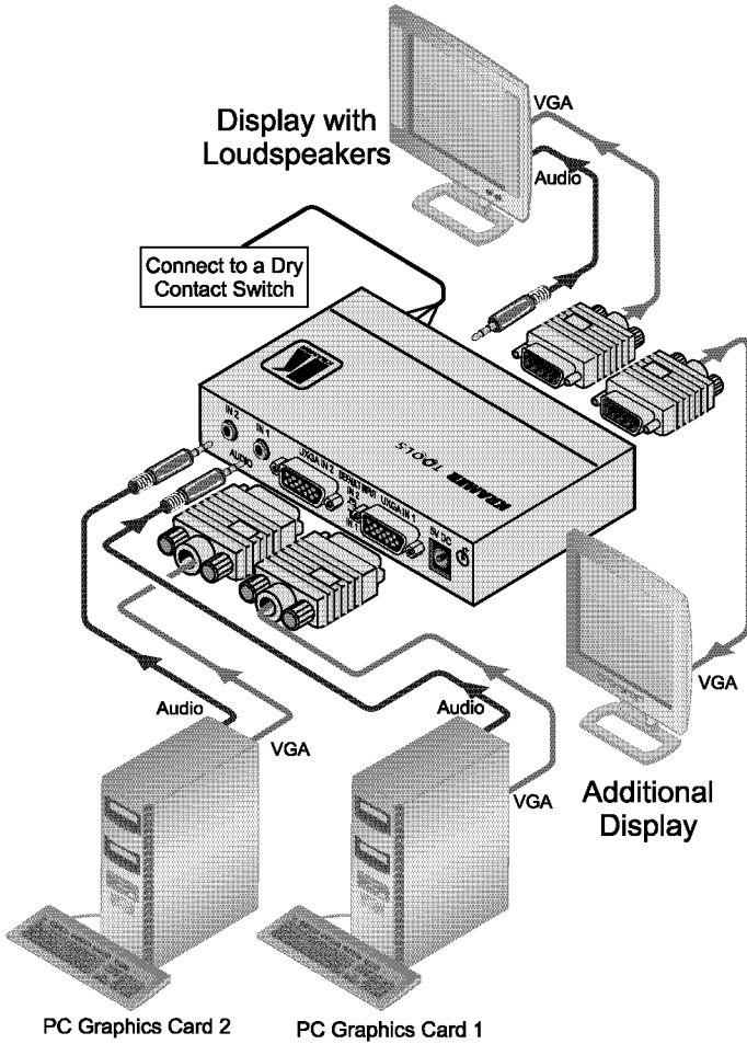
Figure 2: VP-211K Automatic UXGA / Audio Switcher Connections
