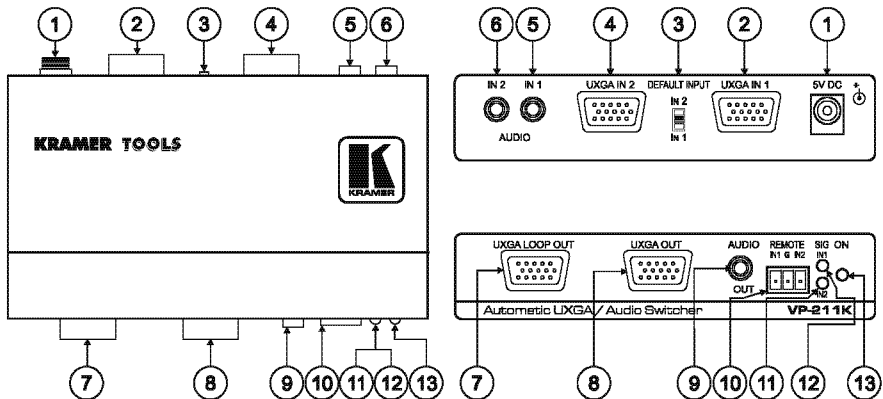
Figure 1: VP-211K Automatic UXGA / Audio Switcher
