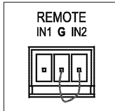
Figure 3: REMOTE Terminal Block Connector
