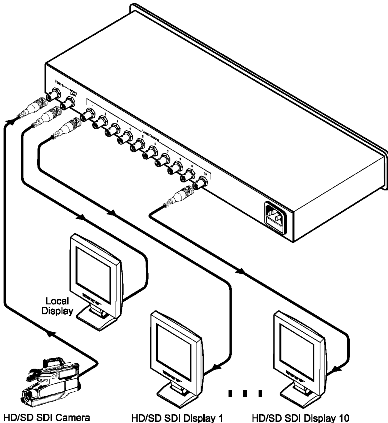
Figure 2: Connecting the VM-10HDxl 3G 1:10 HD/SD - SDI Distribution Amplifier
