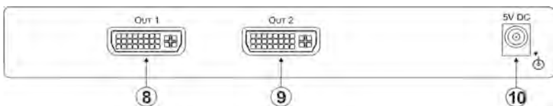
Figure 2: VM-300HDCP 1:3 DVI Distributor Rear Panel
