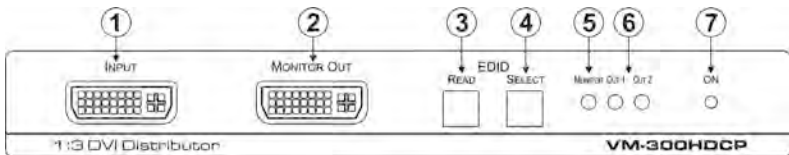
Figure 1: VM-300HDCP 1:3 DVI Distributor Front Panel
