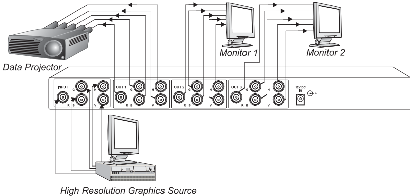
Figure 3: Connecting the VP-123 1:3 RGBHV Distributor
