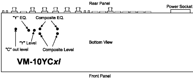
Figure 4: VM-10YCxl Underside
