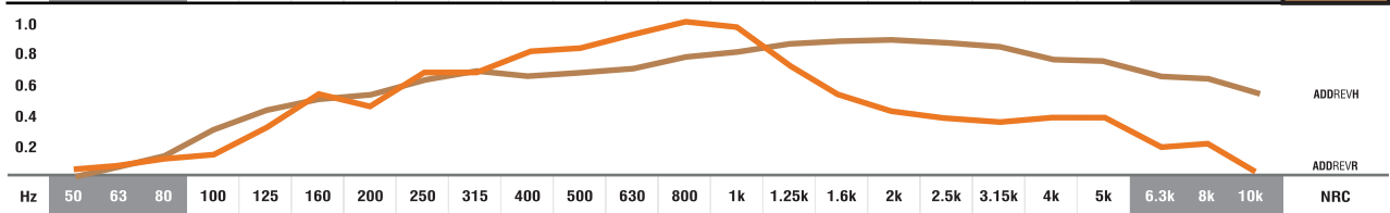
• ● ABSORPTION COEFFICIENT: Values in accordance with the standards: EN 20654, ASTM C423 and EN 11654. ■ Values [<100Hz and > 5K] are Non Standard Values.
