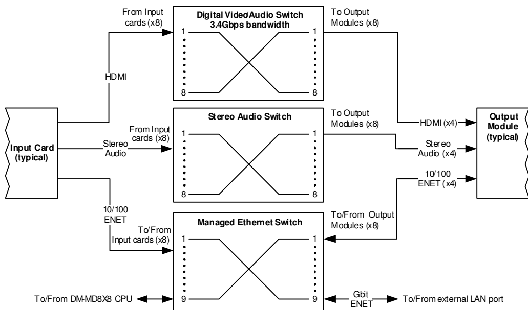
Internal Block Diagram of the DM-MD16X16
