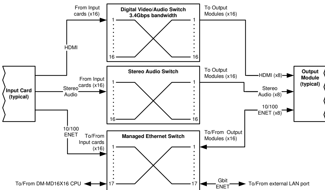
DM-MD16X16 Internal Block Diagram
