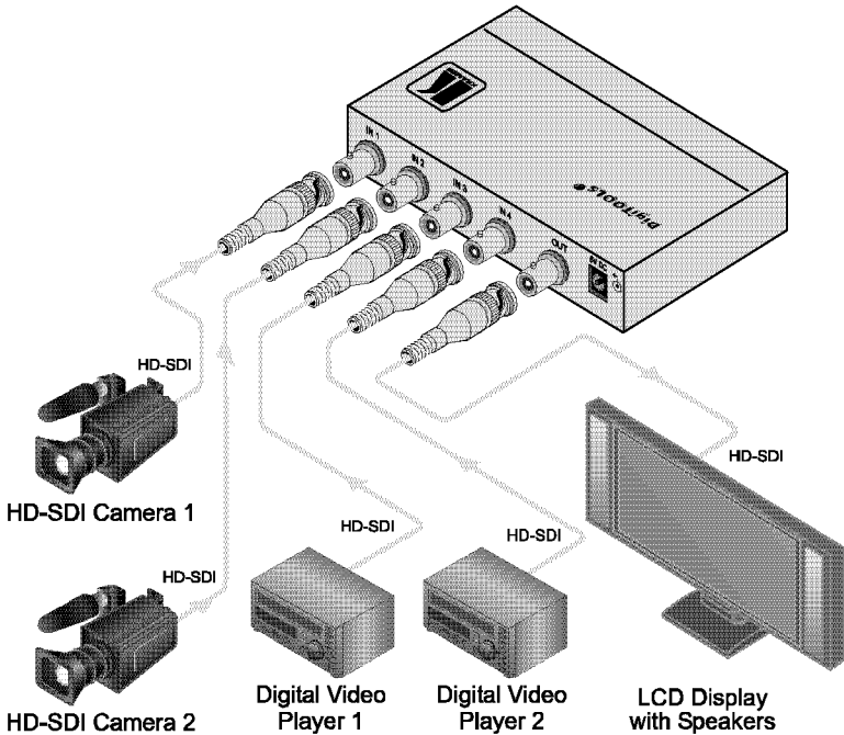
Figure 2: Connecting the 6241HD 4x1 HD-SDI Switcher
