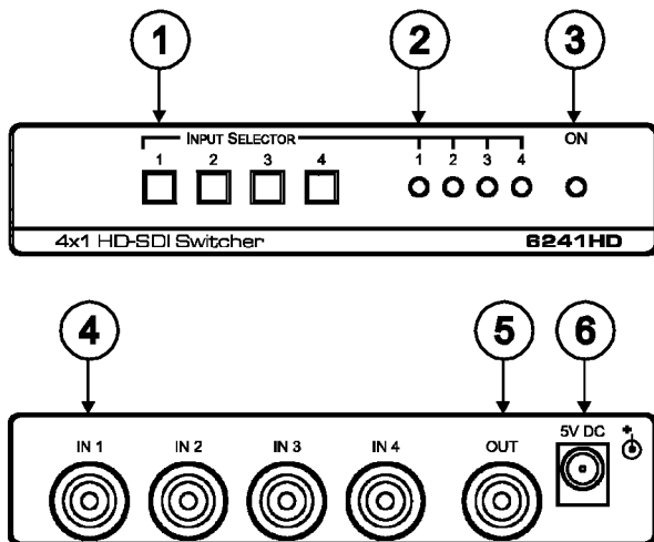
Figure 1: 6241HD 4x1 HD-SDI Switcher Functions
