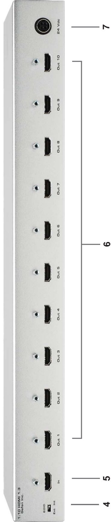
Back Panel
